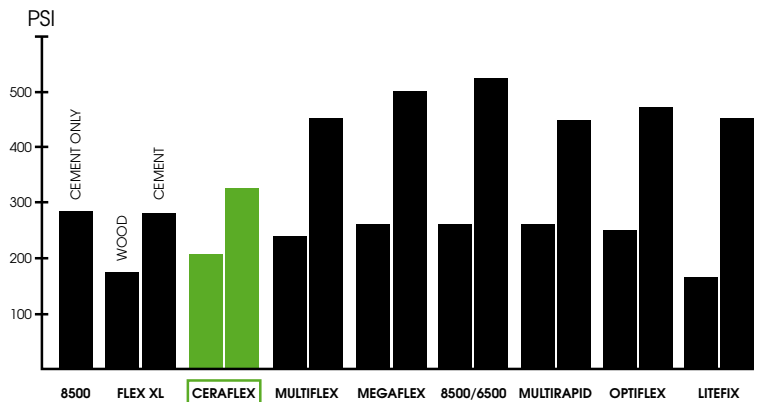
SHEAR STRENGTH COMPARATIVE CHART
